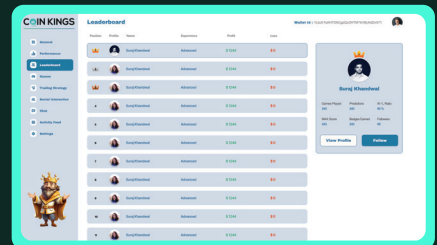
Leaderboard
