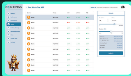
Coin Selection
