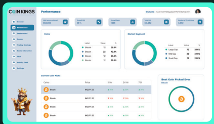
Performance Stats
